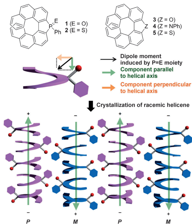
Figure 1. Structures of heterohelicenes and a representation of the columnar packing in a single crystal of rac-2 . Columns with a given dipole moment consist of a single enantiomer ( P or M isomer) and columns with the opposite dipole moment consist of the other enantiomer.
